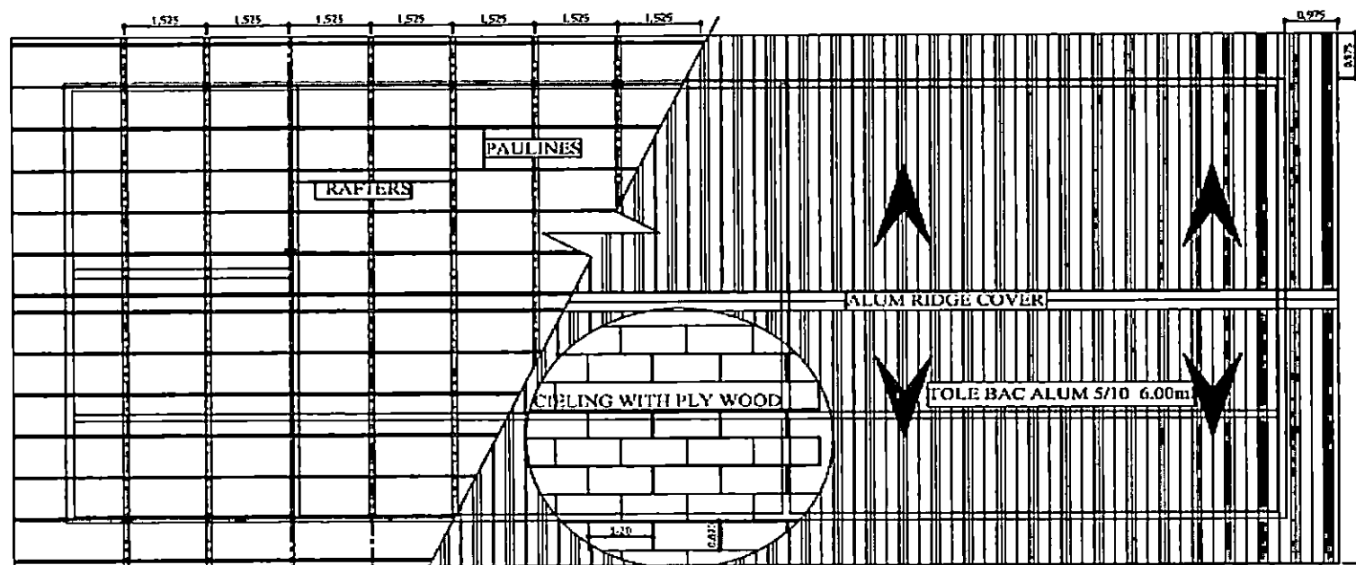
ROOF PLAN
